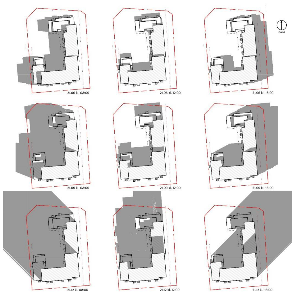
Illustration 12 – Skyggediagrammer
